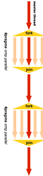
Figure 5. OpenMP is based on a fork-join model
