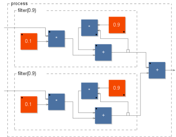
Figure 6. two filters in parallel connected to an adder
