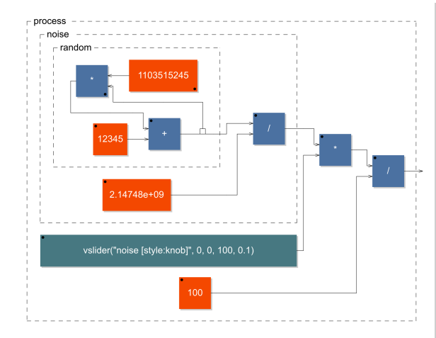
Figure 2. Graphic block-diagram of the noise generator produced with the -svg option
