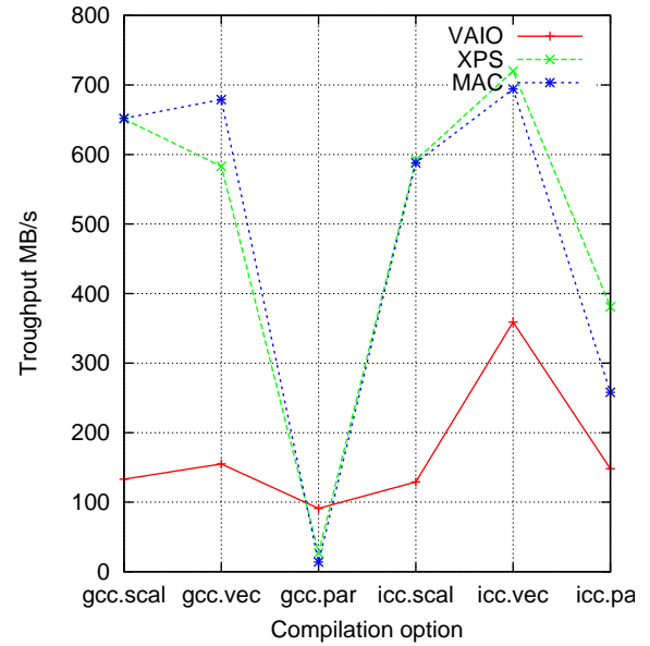
Figure 13. rms.dsp benchmark
