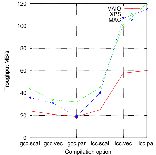
Figure 11. mixer.dsp benchmark
