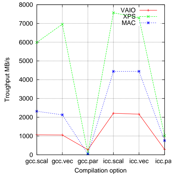
Figure 7. Copy1.dsp benchmark
