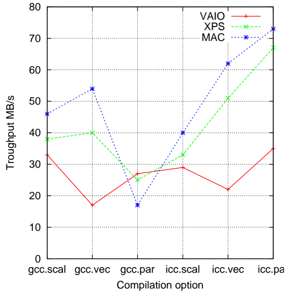
Figure 10. Karplus32.dsp benchmark
