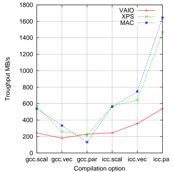
Figure 14. rms8.dsp benchmark
