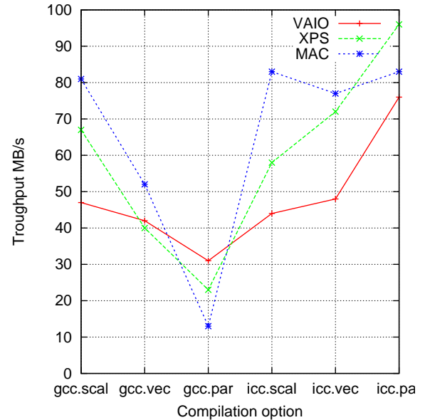
Figure 9. Freeverb.dsp benchmark
