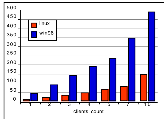
figure 27: service times
